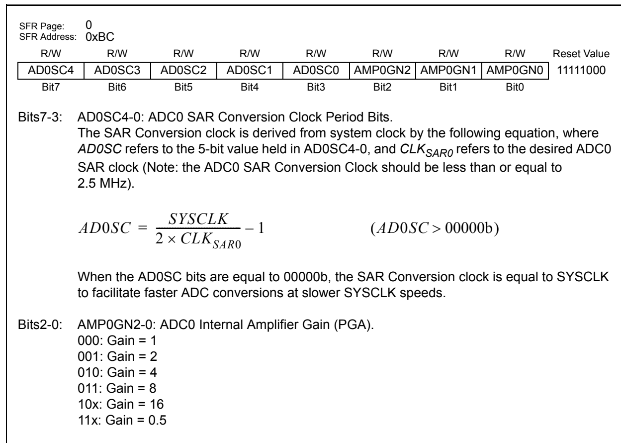
Figure 5.7. ADC0CF: ADC0 Configuration Register
